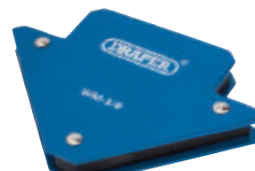
8 WM-3/B MULTI-PURPOSE MAGNETIC HOLDER For holding workpieces whilst soldering or welding. Working angles: 45°, 75° and 135°. Manufactured from high quality pressed and enamelled steel with strong magnet. Display packed.
